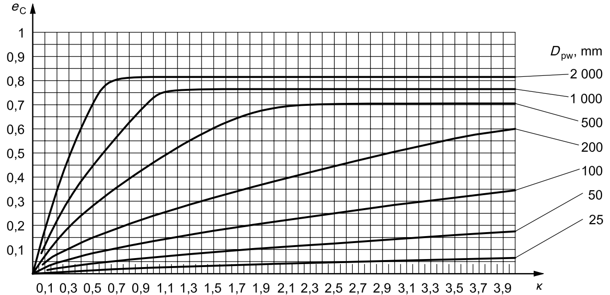
Figure A.3 — e_C factor for circulating oil lubrication with on-line filters — \beta_{25(c)} \geq 75 , ISO 4406 code —/17/14
